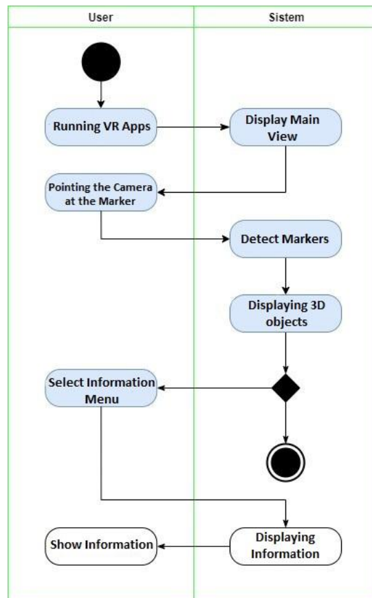
Figure 3: Activity Diagram
