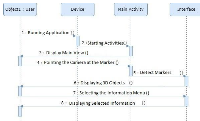
Figure 4: Sequence diagram
